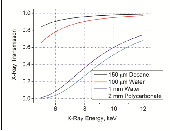
Figure 1: X-ray transmission for various substances vs. x-ray photon energy.
