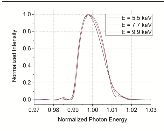
Figure 3: Energy spectrum of the monochromatic x-ray beam for three different average photon energy values. The energy has been normalized by the average energy and the intensity by the peak intensity.
