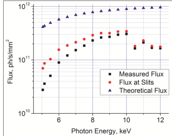
Figure 7. Beamline flux as a function of photon energy.
