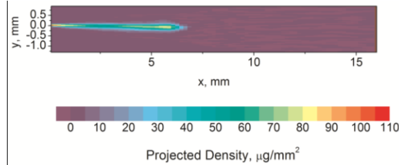
Figure 8. Projected density of a diesel spray 42 \mu\text{s} after the apparent start of injection.
