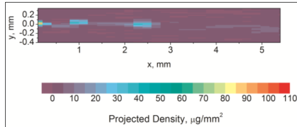
Figure 10. Projected density of dribble in a diesel spray at the end of injection. Note the scale difference compared to Figs. 6 and 7.
