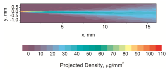
Figure 9. Projected density of a diesel spray 737 \mu\text{s} after the apparent start of injection.
