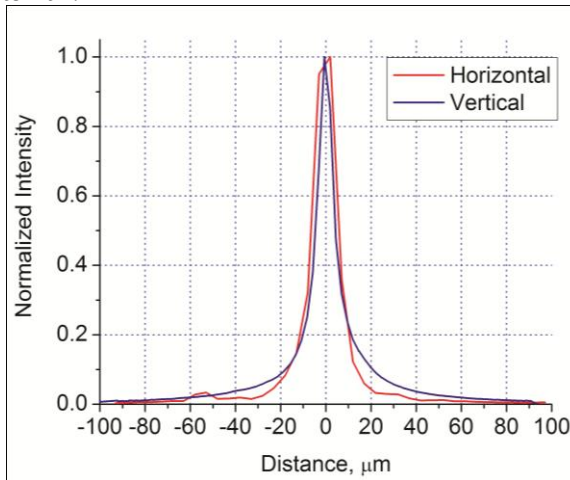
Figure 6. Vertical and horizontal profile of x-ray beam focus as determined by slit scans across the focus spot
