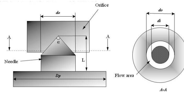
Figure 3. Nozzle configuration
